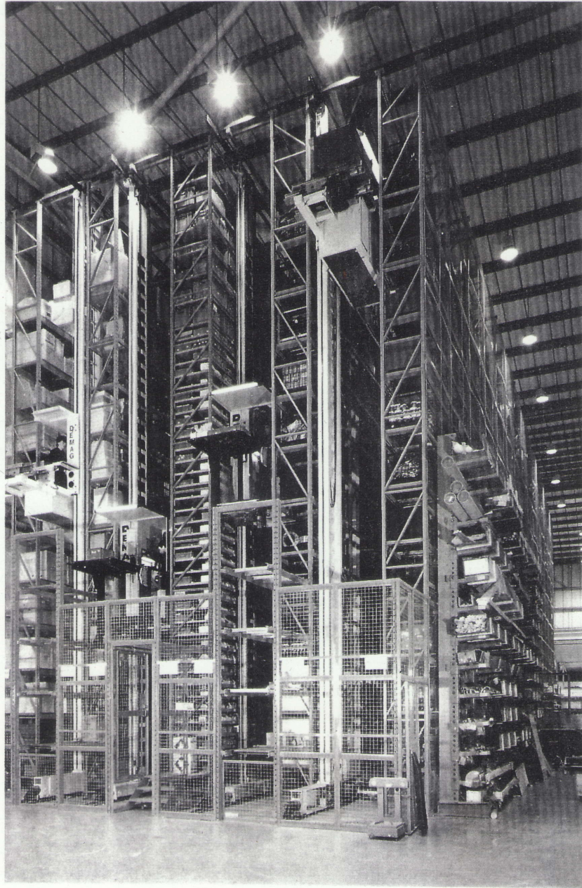
12 Narrow aisle order pickers (By courtesy of Mannesmann Demag Ltd.)
