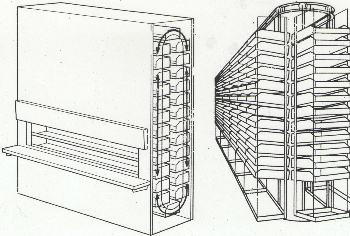
Fig. 30 A vertical and a horizontal carousel
